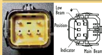
Built-in 6 pin AMP
